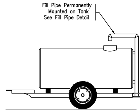
WATER WAGON
