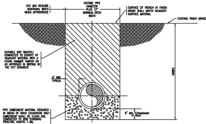
TYPICAL TRENCH SECTION FOR DI PIPE NOT TO SCALE
