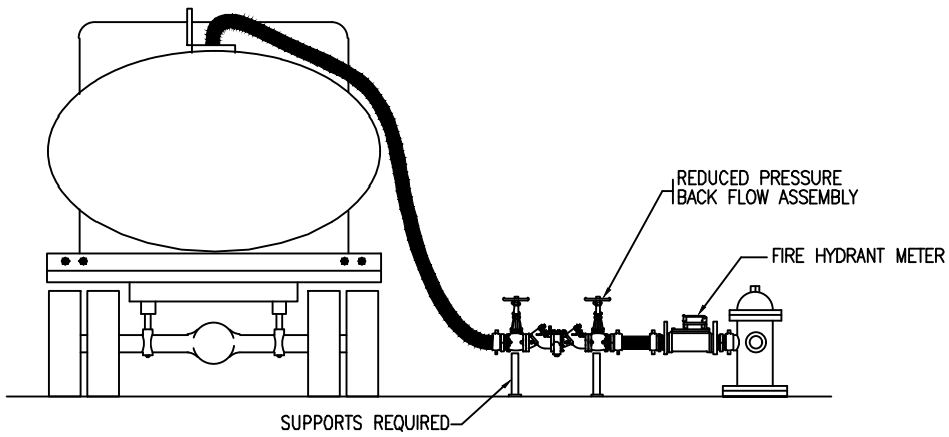
TANK TRUCKS
