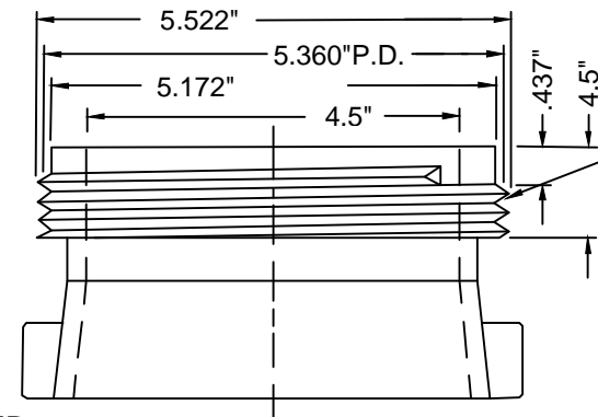
4.5" STEAMER NOZZLE BOARD OF PUBLIC UTILITIES THREAD PATTERN
