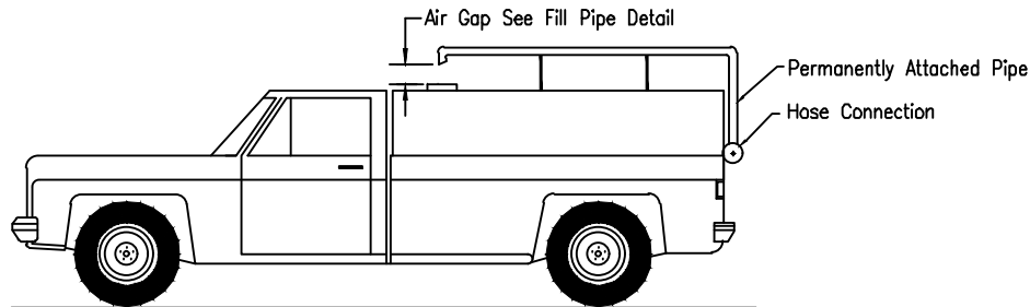
WATER TRUCK
