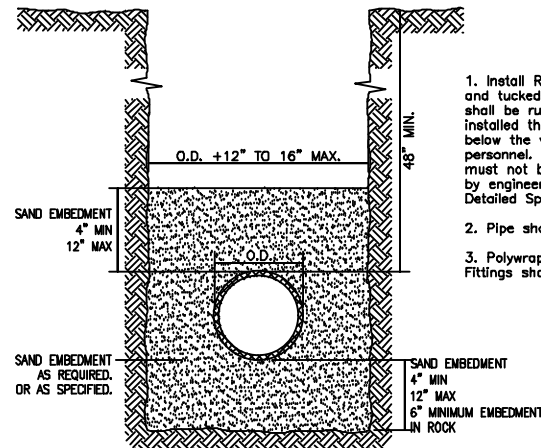
TYPICAL TRENCH SECTION FOR PVC PIPE NOT TO SCALE
