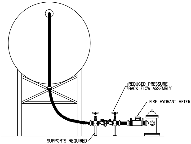
ELEVATED TANK
