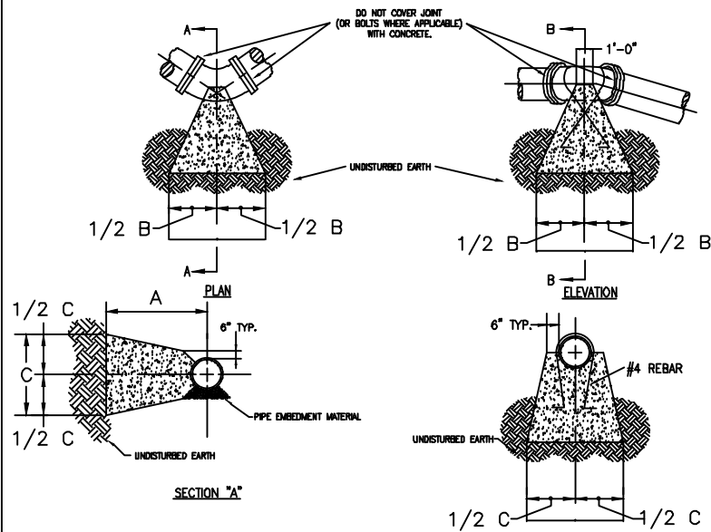
HORIZONTAL THRUST BLOCK DETAILS NOT TO SCALE
