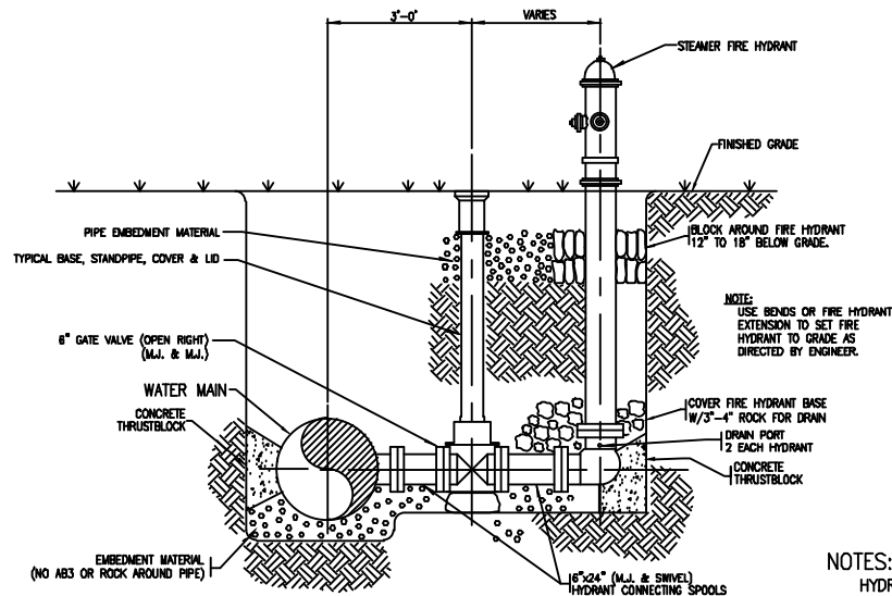
TYPICAL FIRE HYDRANT INSTALLATION NOT TO SCALE
