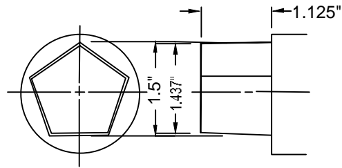
1.5" OPERATING NUT (PENTAGON)
