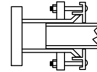
FLANGED CPLG. ADAPTER DETAIL
