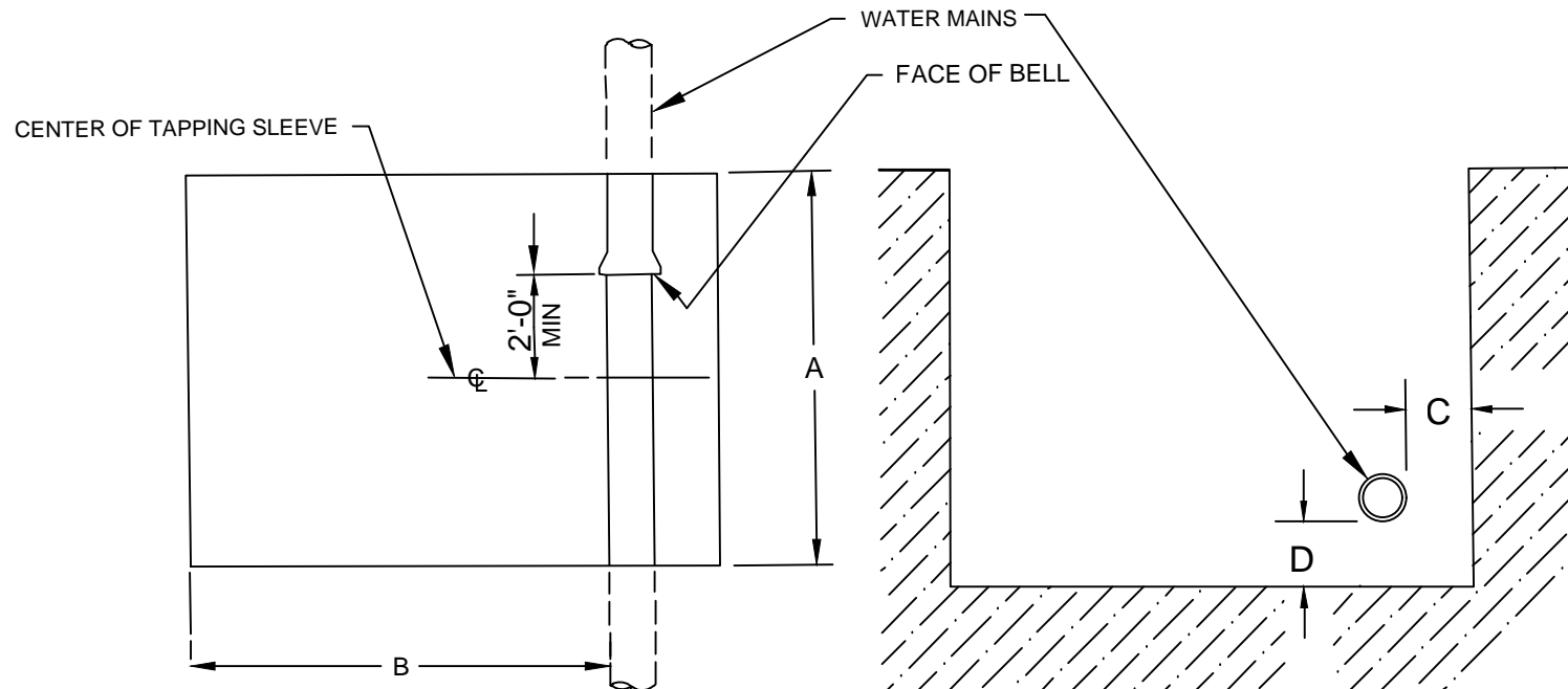
SIZES OF TAP HOLES FOR- 3/4" TO 12" TAPS
