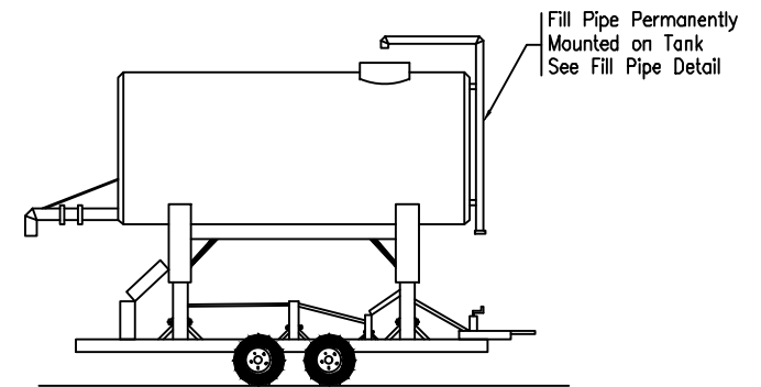
ELEVATED TANK
